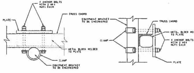
TOP VIEW (TOP CHORD SHOWN, BOTTOM VIEW FOR BOTTOM CHORD)
