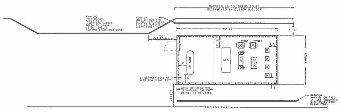
DETAIL 1 EQUIPMENT PLACEMENT AND DIMENSIONS
