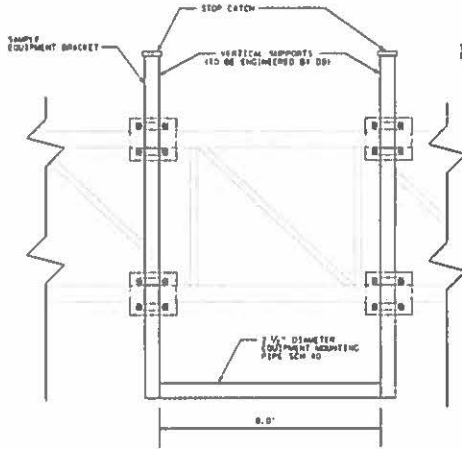
ELEVATION OF GANTRY BRACKET
