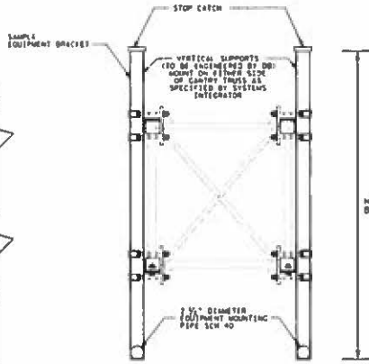
CROSS SECTION OF TOLL GANTRY BRACKET
